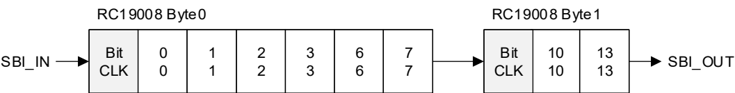
Figure 32. RC19008 Side-Band Shift Order
