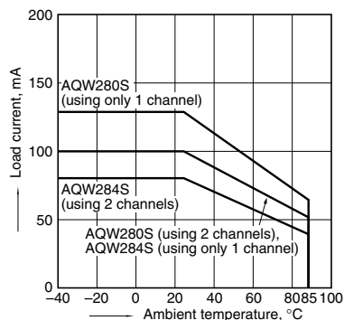
(4) AQW280S, AQW284S
