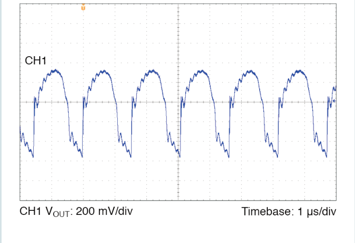
Figure 16 — Output voltage ripple, V_{IN} = 300\text{ V} , V_{OUT} = 24.0\text{ V} , C_{OUT\_EXT} = 1000\text{ }\mu\text{F} , R_{LOAD} = 0.960\text{ }\Omega
