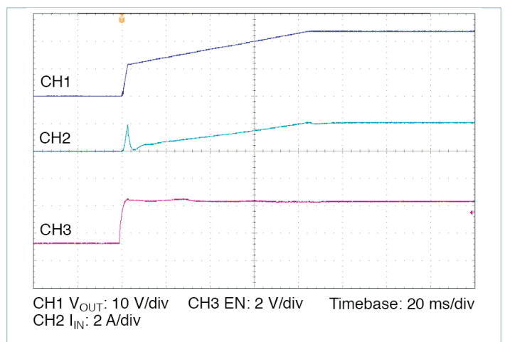
Figure 14 — Startup from EN, V_{IN} = 300\text{ V} , C_{OUT\_EXT} = 10000\text{ }\mu\text{F} , R_{LOAD} = 0.960\text{ }\Omega
