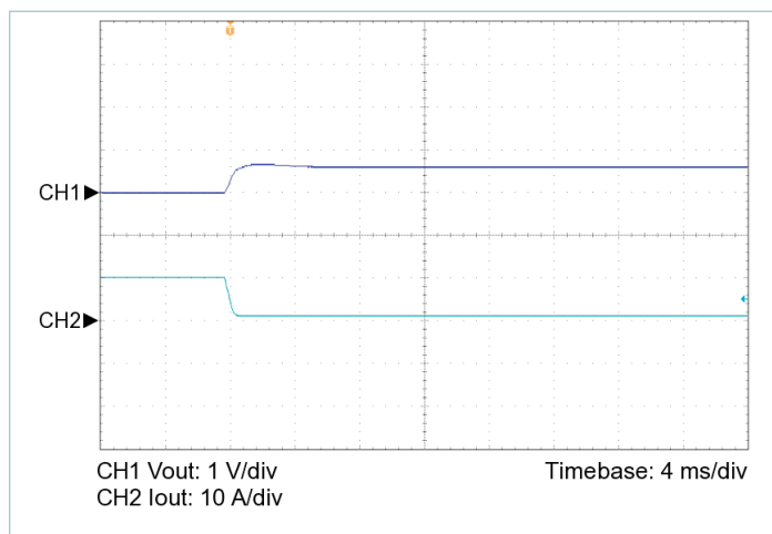
Figure 19 — 100% to 10% load transient response, V_{IN} = 100\text{ V} , nominal trim, C_{OUT\_EXT} = 500\text{ }\mu\text{F}
