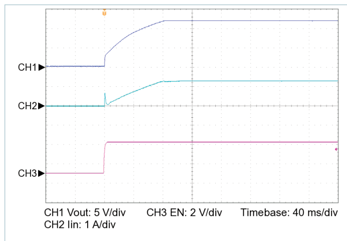
Figure 16 — Startup from EN, V_{IN} = 100\text{ V} , C_{OUT\_EXT} = 10000\text{ }\mu\text{F} , R_{LOAD} = 1.200\text{ }\Omega
