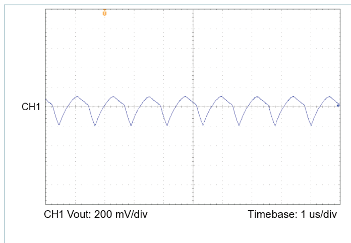
Figure 15 — Output voltage ripple, V_{IN} = 100\text{ V} , V_{OUT} = 12.0\text{ V} , C_{OUT\_EXT} = 500\text{ }\mu\text{F} , R_{LOAD} = 1.200\text{ }\Omega
