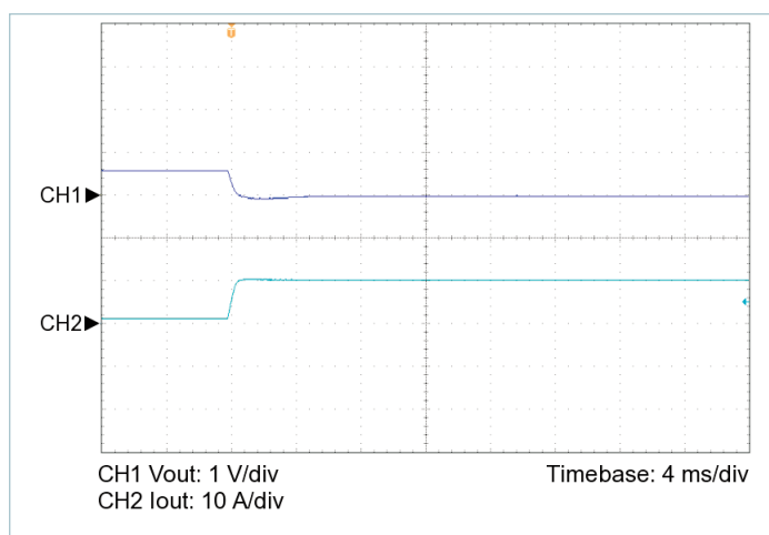
Figure 20 — 10% to 100% load transient response, V_{IN} = 100\text{ V} , nominal trim, C_{OUT\_EXT} = 500\text{ }\mu\text{F}
