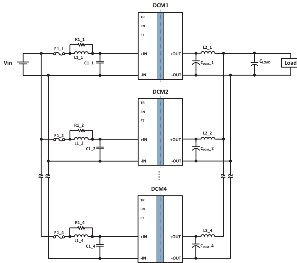
Typical Application 1: DCM4623xD2H31E0yzz in an array of four units
