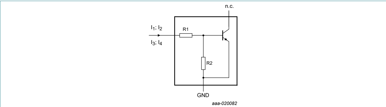
Fig. 10. Resistor test circuit
