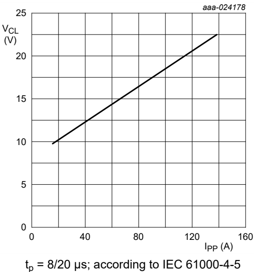
Fig. 10. Positive clamping voltage (8/20 \mu s pulse); typical values
