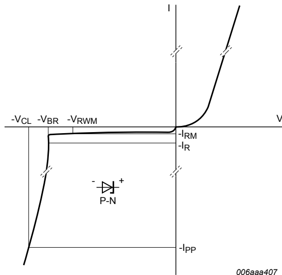
Fig. 8. V-I characteristics for unidirectional ESD protection diode
