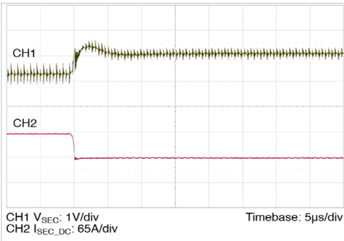
Figure 16 — 62.5A – 0A transient response: C_{\text{PRI\_IN\_EXT}} = 10\mu\text{F} , no external C_{\text{SEC\_OUT\_EXT}}
