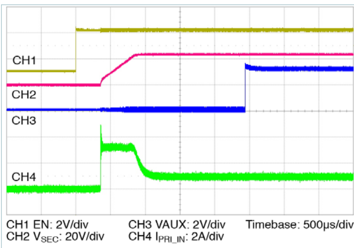
Figure 18 — Startup from application of EN with pre-applied V_{\text{PRI\_DC}} = 384\text{V} , 20% I_{\text{SEC\_OUT\_DG}} , 100% C_{\text{SEC\_OUT\_EXT}}
