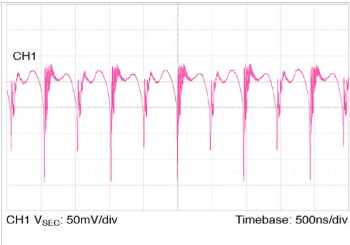
Figure 14 — Full load secondary voltage ripple, 10\mu\text{F} C_{\text{PRI\_IN\_EXT}} ; No external C_{\text{SEC\_OUT\_EXT}} . Board mounted module, scope setting: 20MHz analog BW
