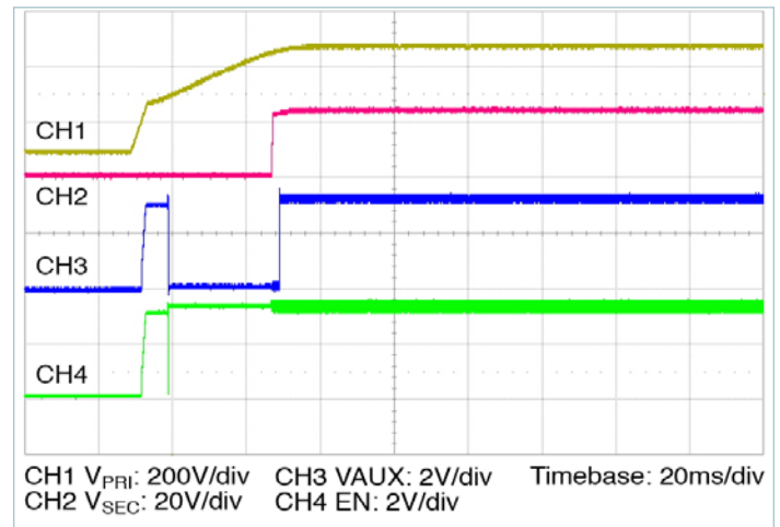
Figure 17 — Startup from application of V_{\text{PRI\_DC}} = 384\text{V} , 20% I_{\text{SEC\_OUT\_DG}} , 100% C_{\text{SEC\_OUT\_EXT}}
