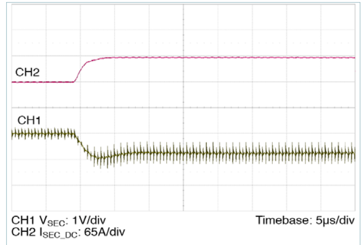
Figure 15 — 0A– 62.5A transient response: C_{\text{PRI\_IN\_EXT}} = 10\mu\text{F} , no external C_{\text{SEC\_OUT\_EXT}}
