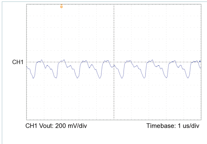
Figure 15 — Output voltage ripple, V_{IN} = 43\text{ V} , V_{OUT} = 15.0\text{ V} , C_{OUT\_EXT} = 1000\text{ }\mu\text{F} , R_{LOAD} = 2.239\text{ }\Omega
