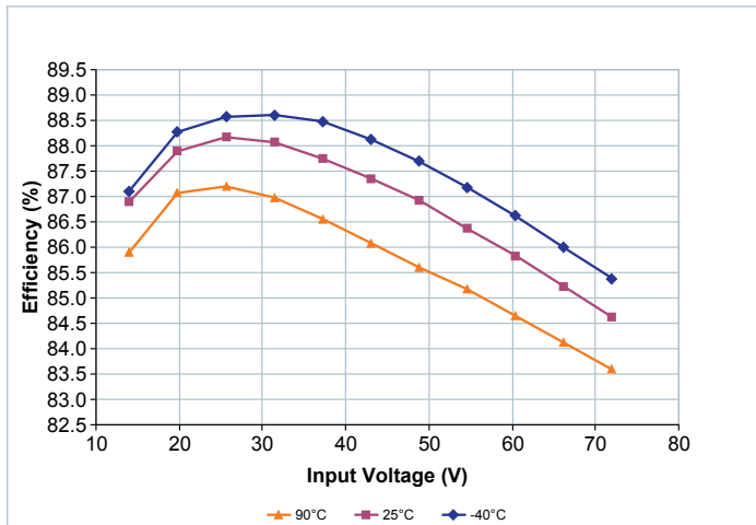
Figure 6 — Full Load Efficiency vs. V_{INL} at low trim
