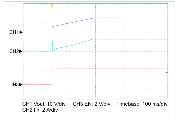
Figure 16 — Startup from EN, V_{IN} = 43\text{ V} , C_{OUT\_EXT} = 10000\text{ }\mu\text{F} , R_{LOAD} = 2.239\text{ }\Omega
