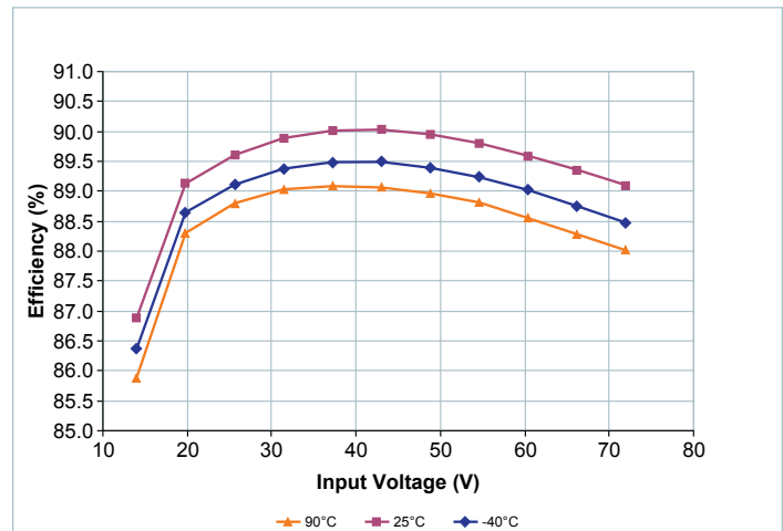
Figure 7 — Full Load Efficiency vs. V_{INL} at nominal trim
