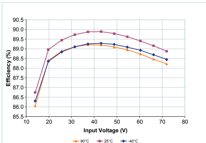
Figure 8 — Full Load Efficiency vs. V_{INL} at high trim
