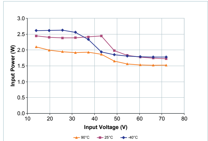
Figure 5 — No load power dissipation vs. V_{INL} at nominal trim
