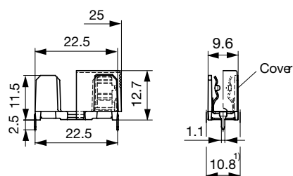
1) Installation dimension
