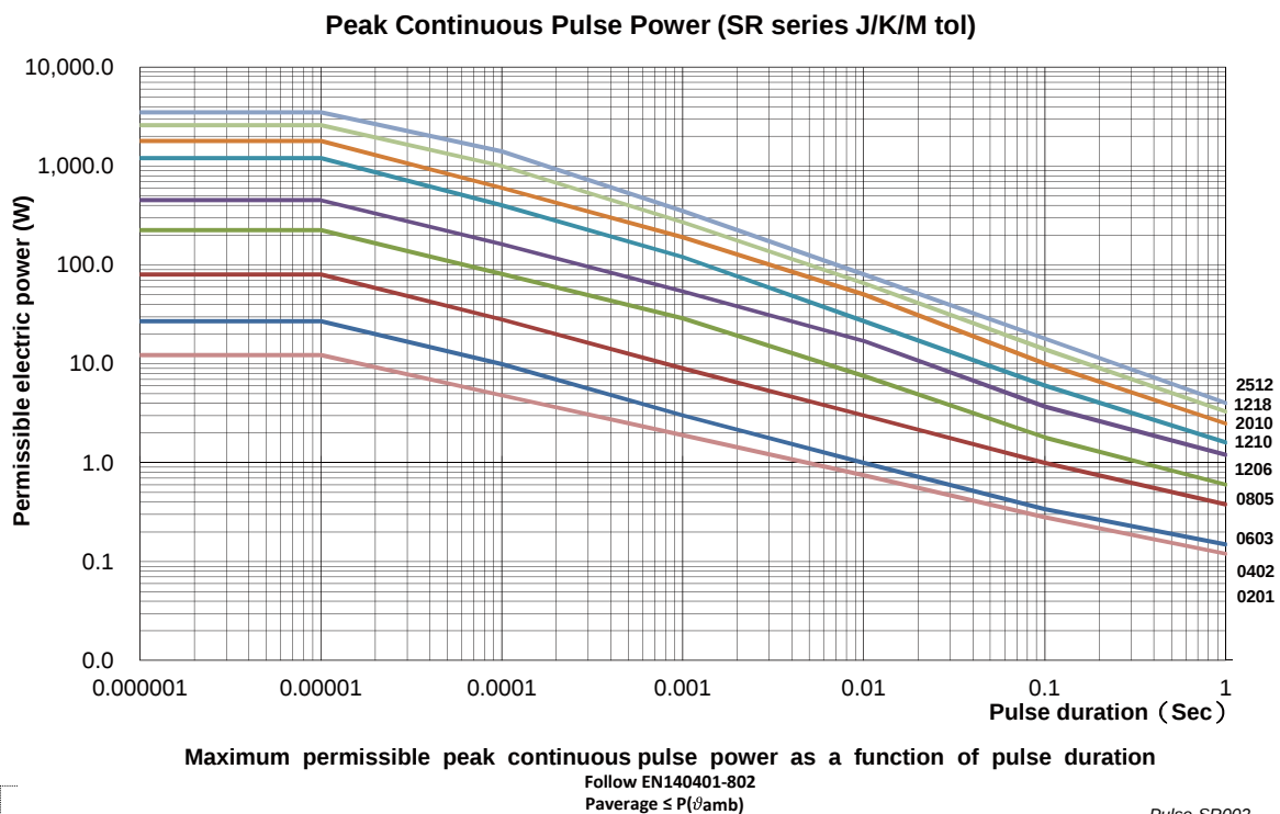
Fig. 7-4 Pulse-Load behavior
