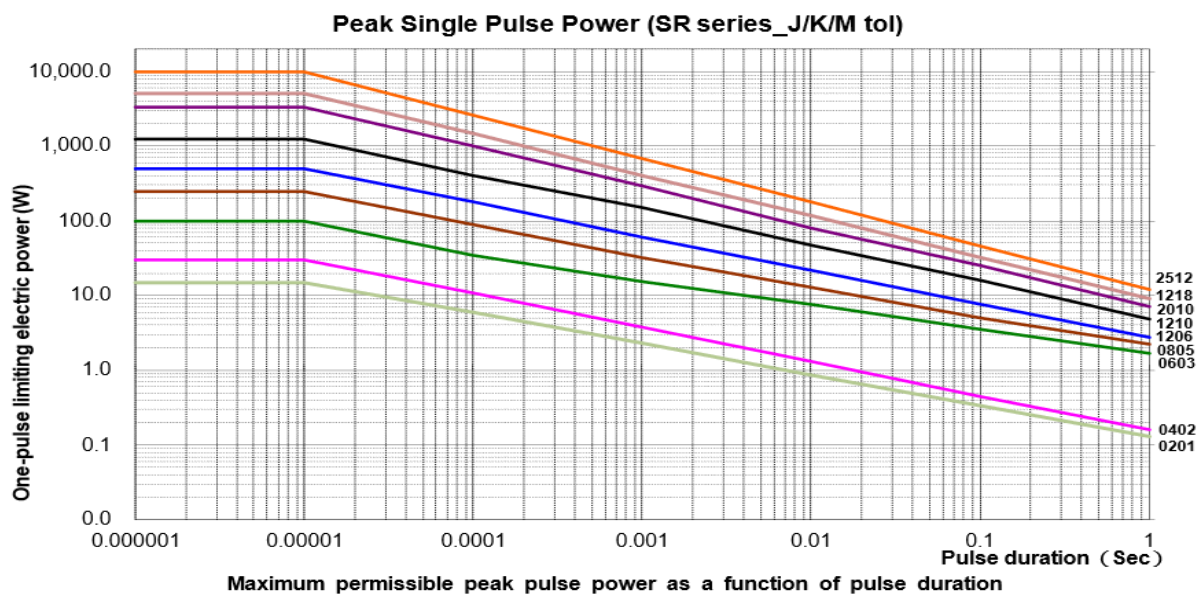
Fig. 7-2 Pulse-Load behavior
