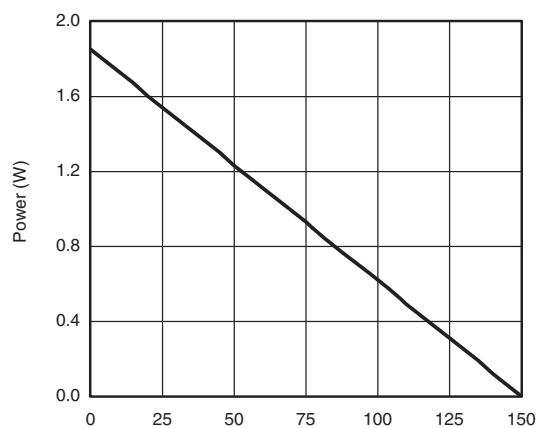
Power, Junction-to-Ambient
