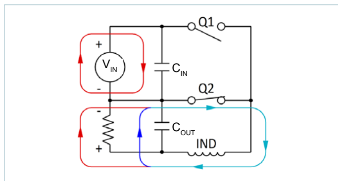
Figure 64 — Current flow: Q2 closed
