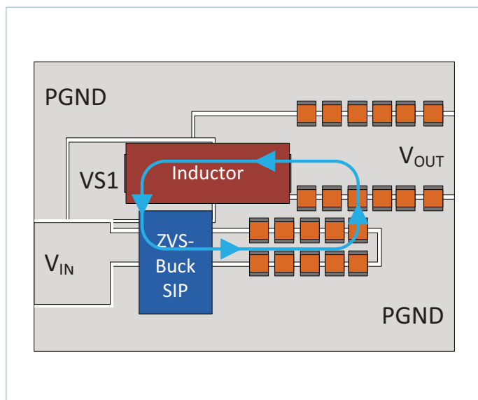
Figure 65 — Recommended layout for Optimized AC Current within the SIP, Inductor, and Ceramic Input and Output Capacitors
