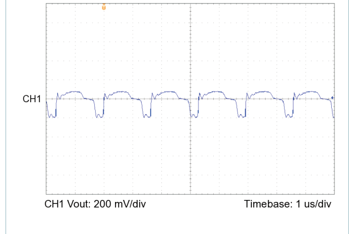
Figure 16 — Output voltage ripple, V_{IN} = 30\text{ V} , V_{OUT} = 5.0\text{ V} , C_{OUT\_EXT} = 1000\text{ }\mu\text{F} , R_{LOAD} = 0.313\text{ }\Omega
