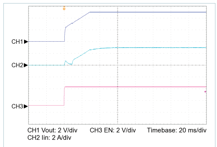
Figure 14 — Startup from EN, V_{IN} = 30\text{ V} , C_{OUT\_EXT} = 10000\text{ }\mu\text{F} , R_{LOAD} = 0.313\text{ }\Omega
