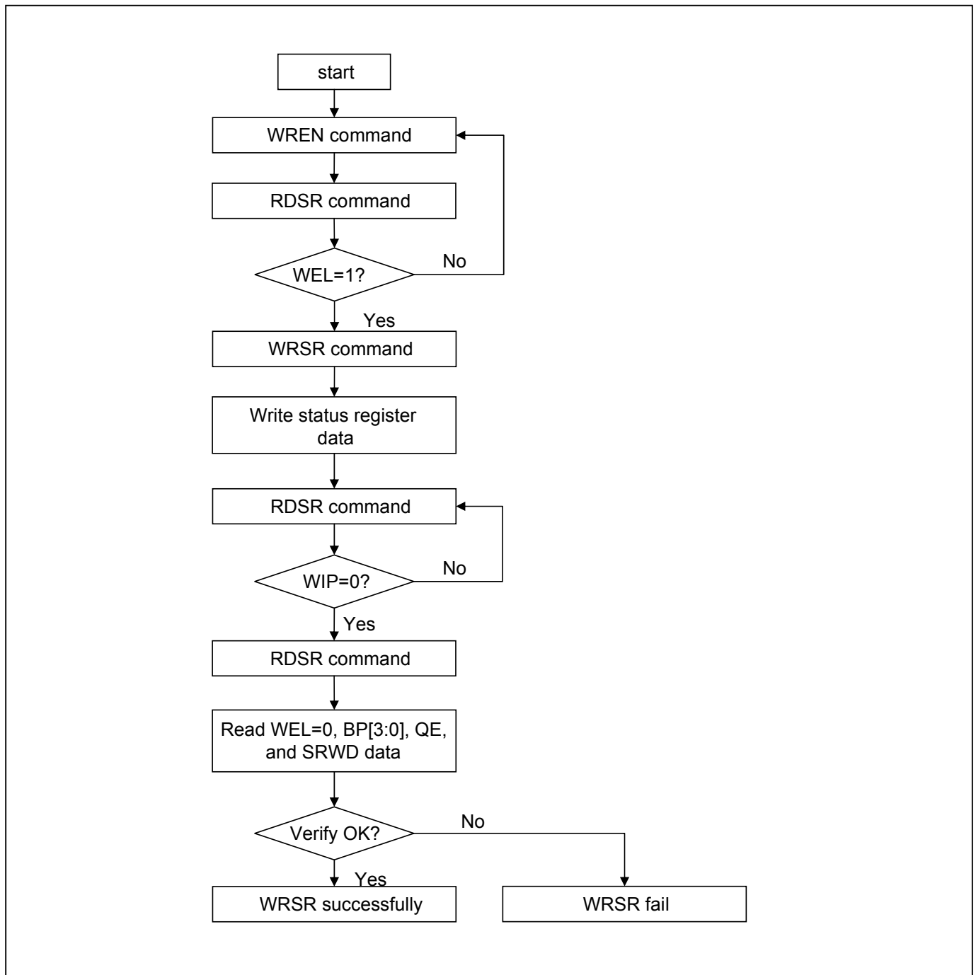
Figure 16. WRSR flow
